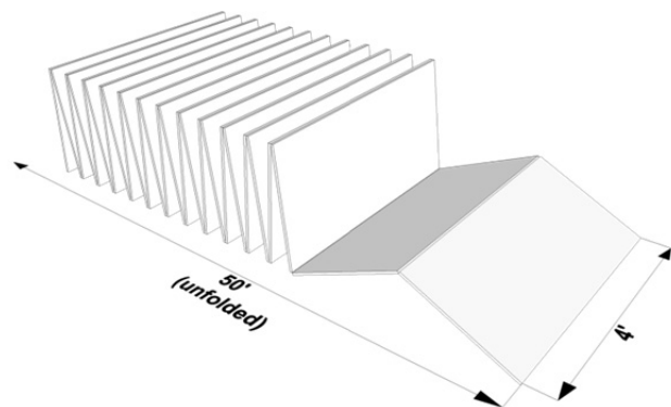
Figure 2. Duro-Guard XPS Fan Fold – P Dimensions
